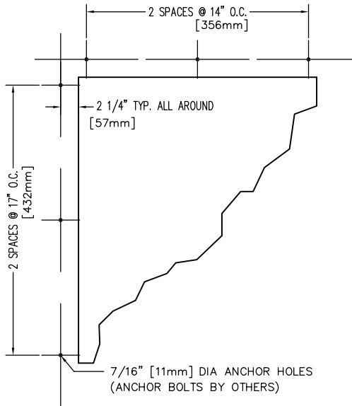
ANCHOR HOLE LAYOUT
